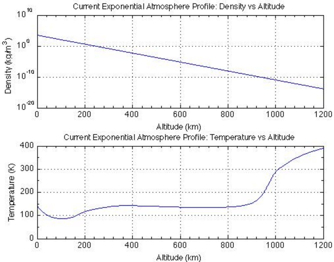
Figure 8-10 Saturn_Longuski Atmosphere
