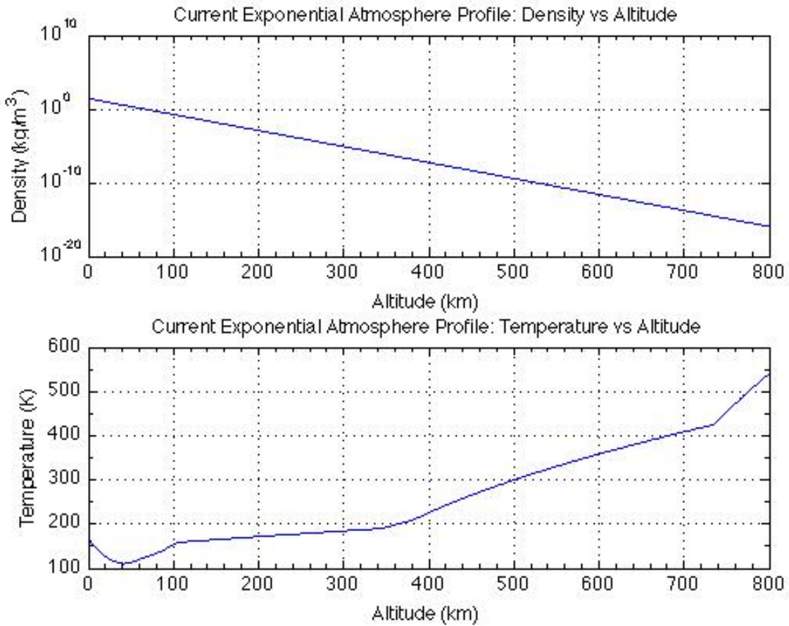
Figure 8-9 Jupiter_Longuski Atmosphere
